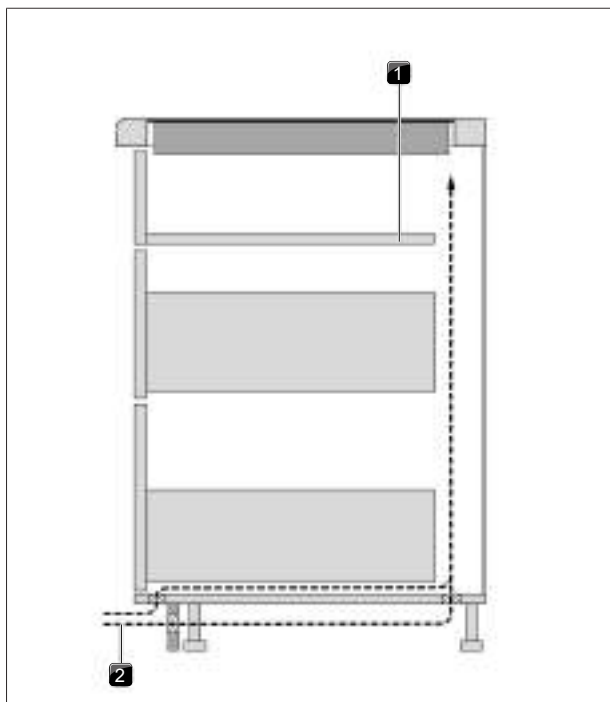
Fig. 4.7 Plinth area air supply
